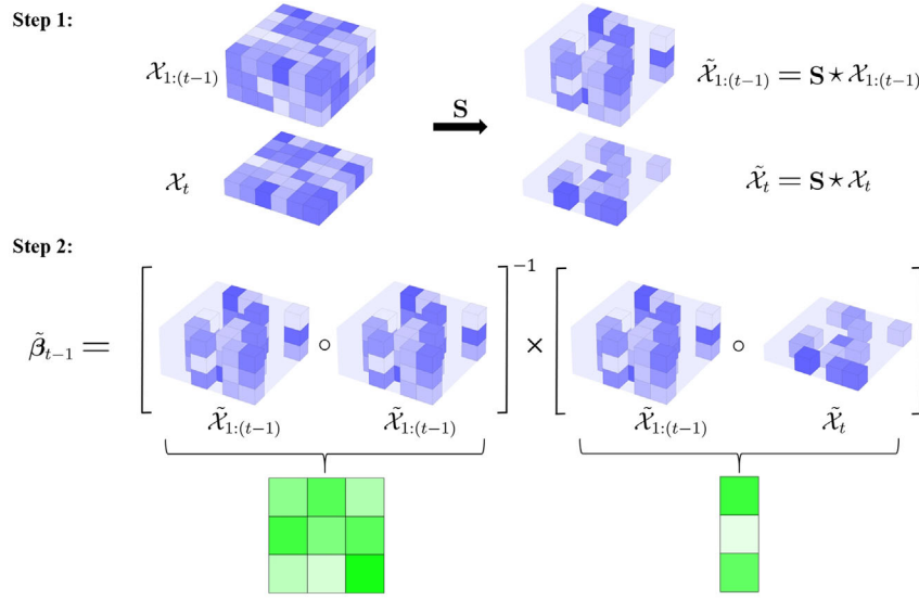
Figure 2. An illustration of parameter approximation by subsampling. The nonzero elements of each tensor(matrix, vector) are labeled with non-transport colors. Step 1 illustrates the subsampling process through mask \mathbf{S} . Step 2 illustrates the parameter approximation.
